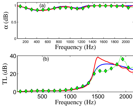
Figure 5. Results for the absorption (a) and the transmission loss (b) for the ABH muffler predicted using TMM (blue), FEM (red) and measured on the experimental set-up (green).
