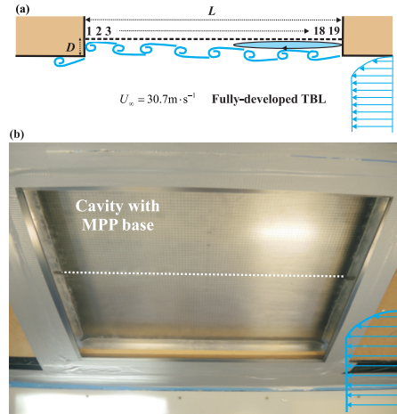
Fig. 2. (a) sketch of a transitional flow cavity with micro-perforated base wall beneath a fully developed turbulent boundary layer; (b) photograph of the wind tunnel test section on top of which is mounted the micro-perforated cavity: the white points over the cavity base correspond to the 19 wall-pressure measurements positions ordered as indicated in Fig. 2(a).
